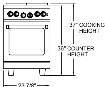
OVERALL WIDTH
